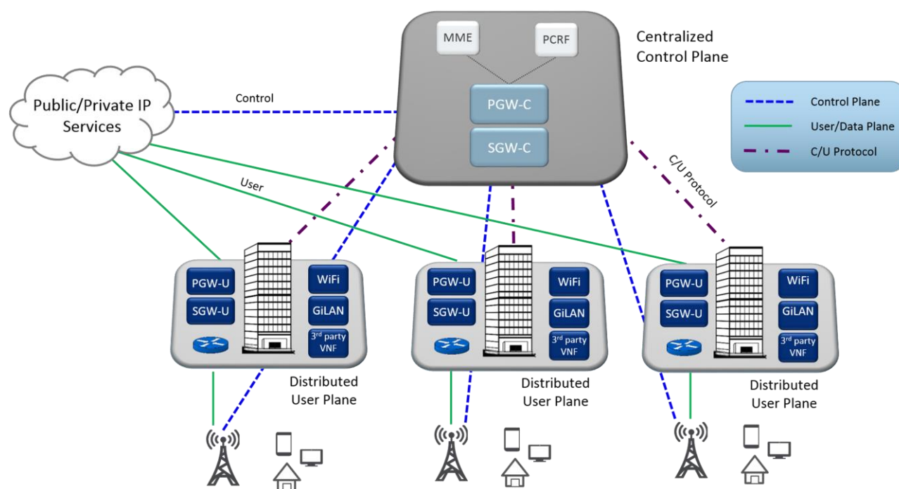
Figure 10: Distributed User-Plane at Edge Data Centers
