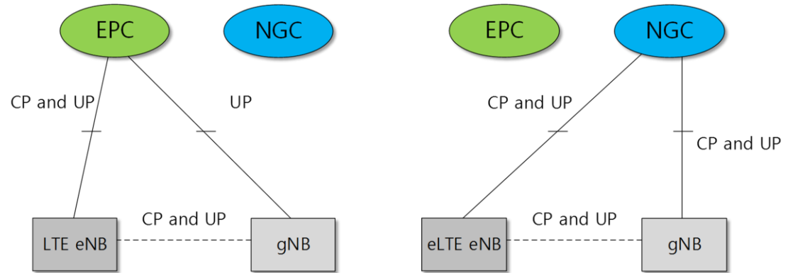
Figure 4: Migrating 5G RAN from EPC to NG Core
